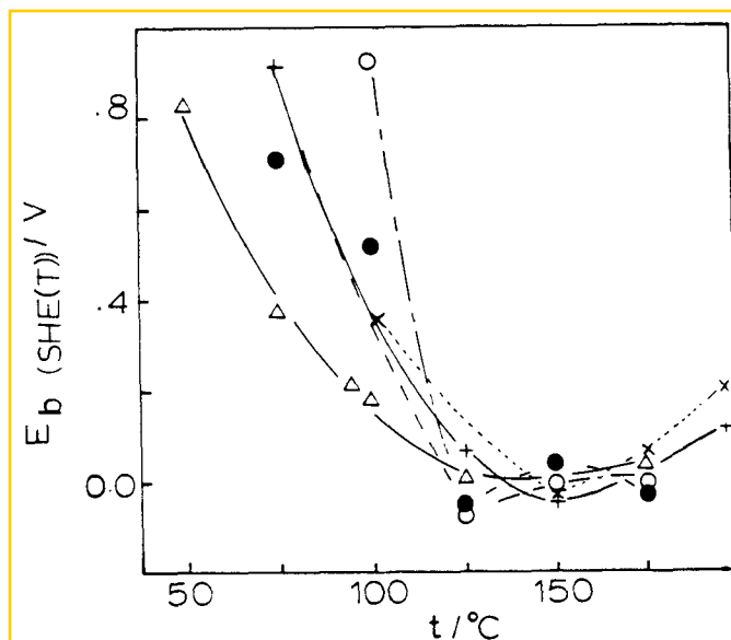
FIGURE 4 — Passivation breakdown potentials: (+) Alloy 625, 0.1% NaCl, (Δ) Alloy 625, 20% NaCl, (●) Alloy C-276, 20% NaCl, (○) Alloy C-276, 1% NaCl, and (X) Alloy C-276, 0.1% NaCl.
